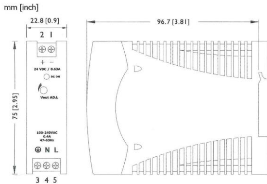
DPP15-24 Dimensions
